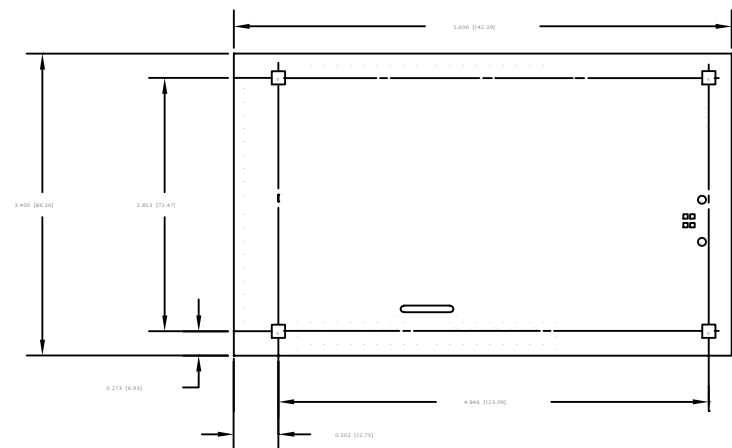
PCB DIMENSIONS AND HOLE LOCATIONS
